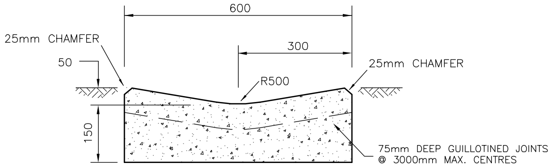
OPEN INVERT CROSSING (TO INTERSECT WITH SEMI-MOUNTABLE (MODIFIED) KERB & CHANNEL)
