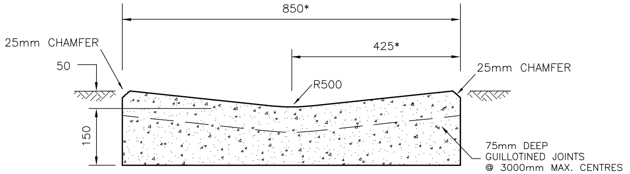
OPEN INVERT CROSSING (TO INTERSECT WITH 600-WIDTH BARRIER KERB & CHANNEL)
