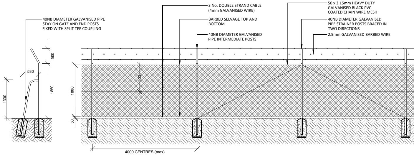
01 POST AND STARINER POSTS ASSEMBLY - SECTION SCALE: 1:75 @ A4
