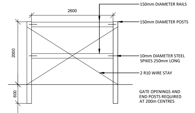
05 STRAINING POST ASSEMBLY - SECTION SCALE: 1:75 @ A4
