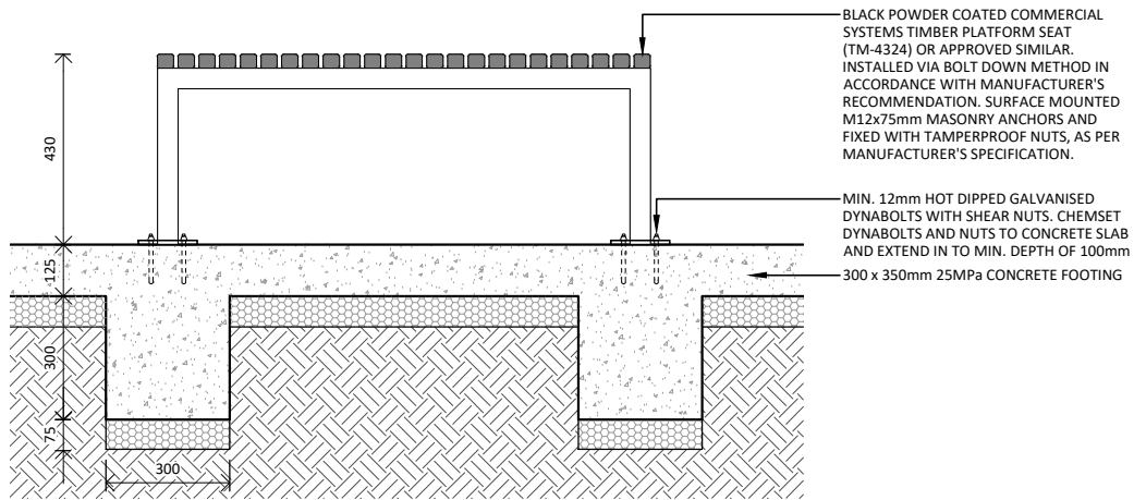
01 TIMBER PLATFORM SEAT - SECTION SCALE: 1:20 @ A4
