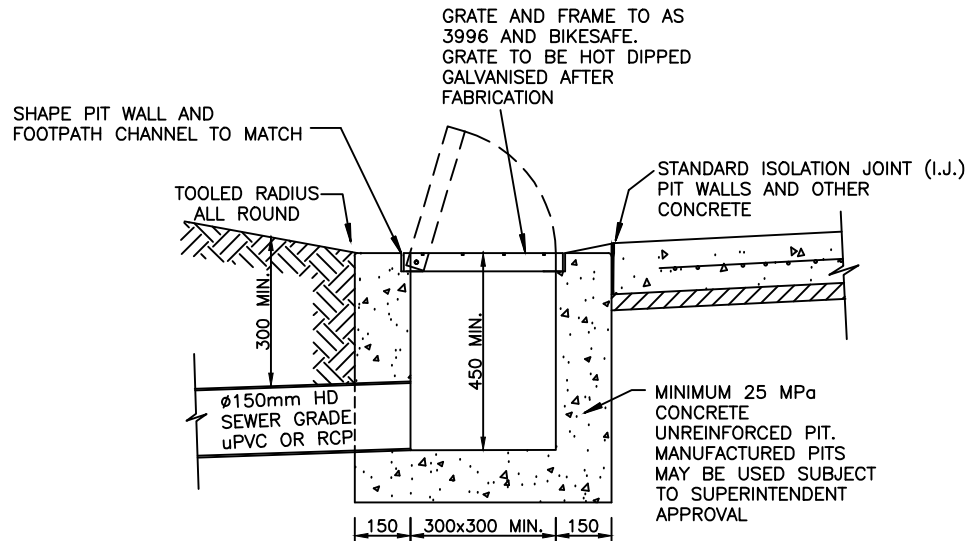
FOOTPATH GRATING PIT DETAIL
