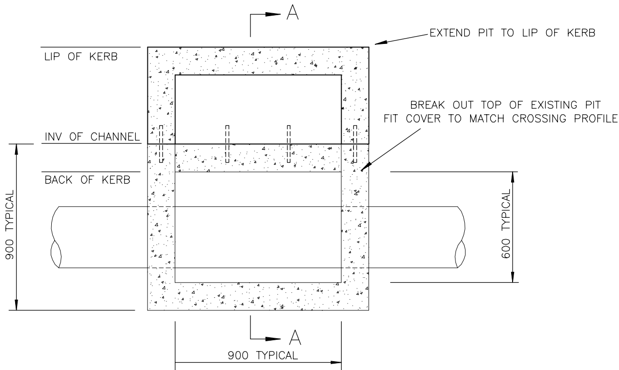
PLAN (COVER, GRATE & FRAMES REMOVED)
