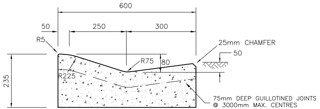
SM2(Mod) – SEMI-MOUNTABLE (MODIFIED) KERB & CHANNEL
