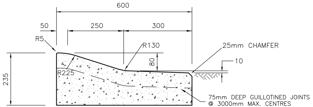
SM3(Mod) – SEMI-MOUNTABLE (MODIFIED) KERB & OUTFALL TRAY
