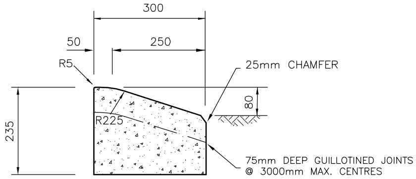
SM1(Mod) – SEMI-MOUNTABLE (MODIFIED) KERB
