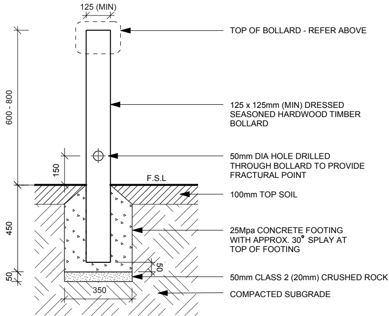
SECTION - FRANGIBLE TIMBER BOLLARD
